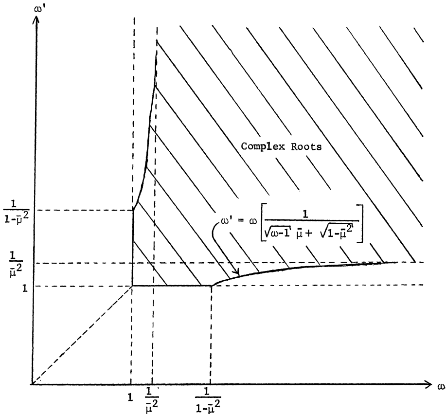
FIGURE 5.1. Regions of Real and Complex Eigenvalues of \mathcal{S}_{\omega, \omega'} .
